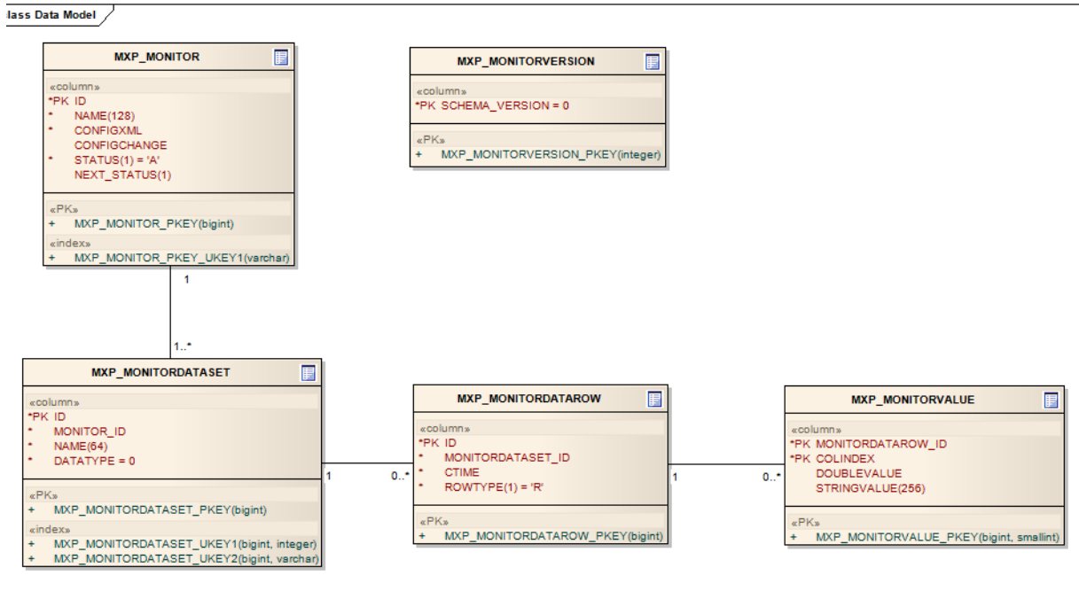
Figure 15: DB monitor data model.
