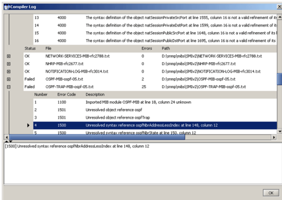
Figure 1: Compiler Log window with compilation errors displayed per MIB module.
